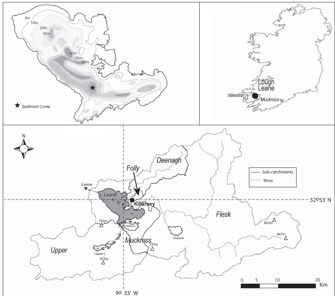
Fig. 1 —Location map, showing Lough Leane and its catchment in southwest Ireland. Also shown are the boundaries of the four subcatchments (including that of the Folly stream) and the main rivers draining into and out of the lake, bathymetric variations (including the deepest point coring site), and the location of the meteorological stations at Muckross and Valentia.
