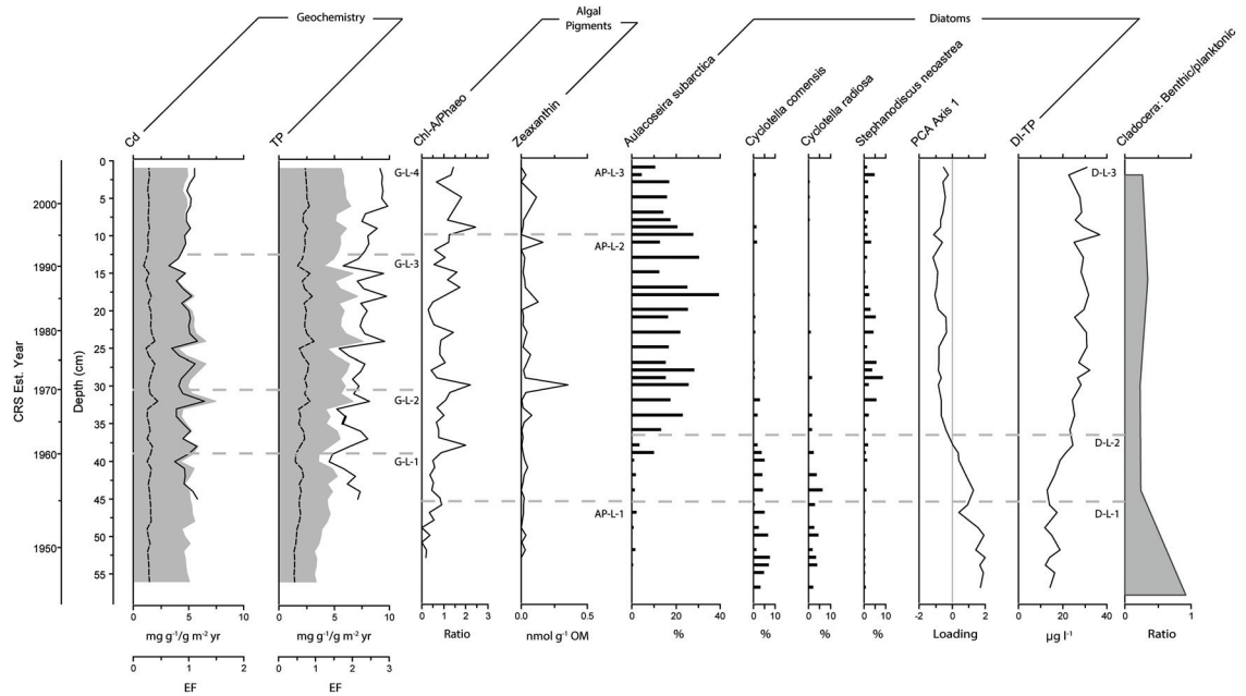
Fig. 4 —Summary plot showing the key changes in the multiproxy palaeolimnological (sedimentary) data collected from Lough Leane. Up-core variations in (from left to right): concentrations (dashed line), accumulation rates (solid line) and EFs (grey silhouettes) for geochemical data; algal pigment data (ratio of chl-a to phaeophytin and zeaxanthin); diatom remains expressed as relative abundances (%), ordination (principal components analysis (PCA) axis 1 sample scores and diatom-inferred total phosphorus (DI-TP)); ratio of benthic–planktonic Cladocera.
