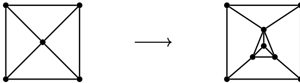
Fig. 7 A vertex-to- K_4 substitution at the center vertex of the wheel graph on 5 vertices. This graph operation will preserve rigidity in any non-Euclidean 2-dimensional normed space [6, Lemma 5.5]
