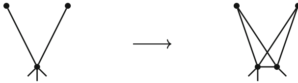
Fig. 5 A 3-dimensional vertex split
