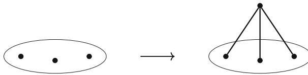
Fig. 3 A 3-dimensional 0-extension
