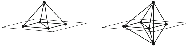
Fig. 2 Left: a coning operation applied to K_4 - e . Right: a bracing operation applied to K_4 - e
