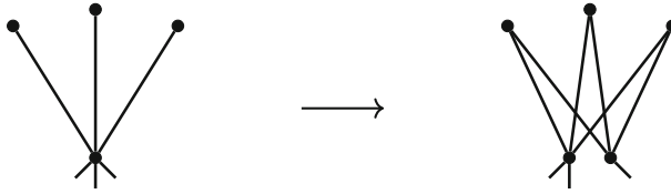
Fig. 6 A 3-dimensional spider split
