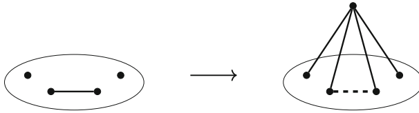
Fig. 4 An example of a 3-dimensional 1-extension
