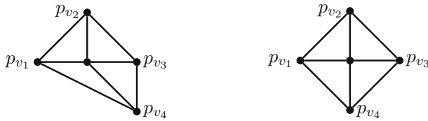
Fig. 1 A bar-joint framework in \ell_q^2 which is regular and minimally rigid (left) and a bar-joint framework which is non-regular (right), for q \in (1, \infty) , q \neq 2
